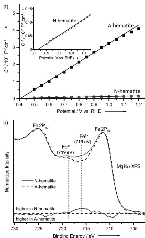
Figure 3. a) Mott–Schottky plots measured for A-hematite (■) and N-hematite (●) nanowire films. The x intercepts of the linear best-fit lines were used to estimate the flat-band potential ( V_{\text{FB}} ). Inset: magnified Mott–Schottky plot of N-hematite. b) Overlay of Fe 2p XPS spectra of A-hematite (----) and N-hematite (—) films, together with their difference spectrum (“N-hematite” minus “A-hematite”). The vertical dashed lines highlight the satellite peaks for \text{Fe}^{3+} and \text{Fe}^{2+} .
