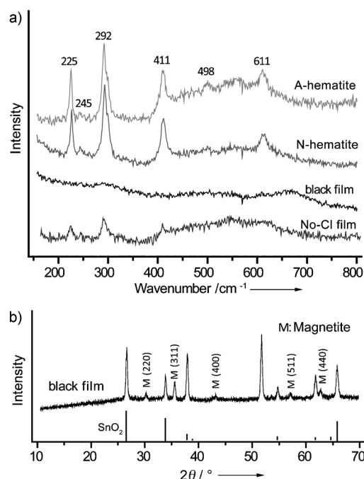
Figure 4. a) Raman spectra of akaganeite samples: thermally treated in air (A-hematite), oxygen-deficient (N 2 + air; N-hematite), N 2 environments (black film), and prepared by a Fe(NO 3 ) 3 precursor solution and thermally treated in N 2 (No-Cl film). b) XRD spectrum collected for the akaganeite samples thermally treated in N 2 at 550 °C. Diffraction peaks labeled with M(hkl) can be indexed to magnetite (JCPDS 19-0629). The lines at the bottom indicate the diffraction peaks of SnO 2 (JCPDS 41-1445) from the FTO substrate.
